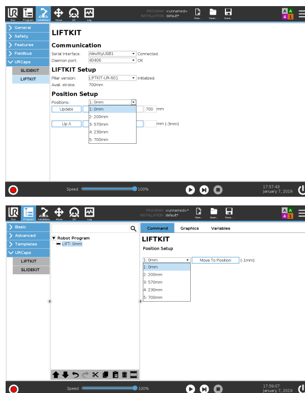
LIFTKIT software functionality
